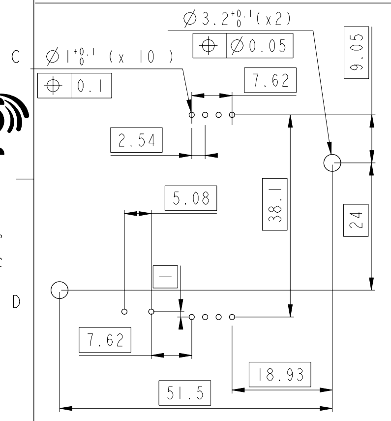
Recommended PCB Layout (Component side)
